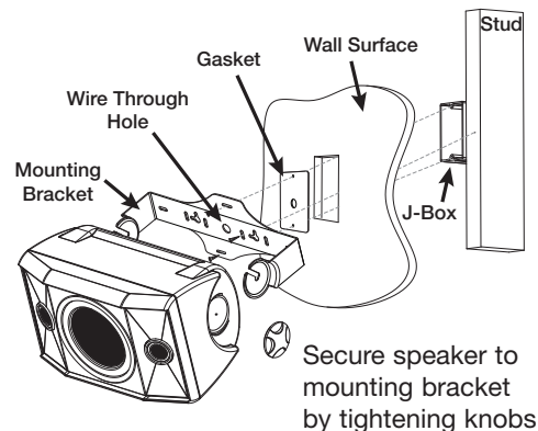
Diagram 4: Pre-Construction Installation
